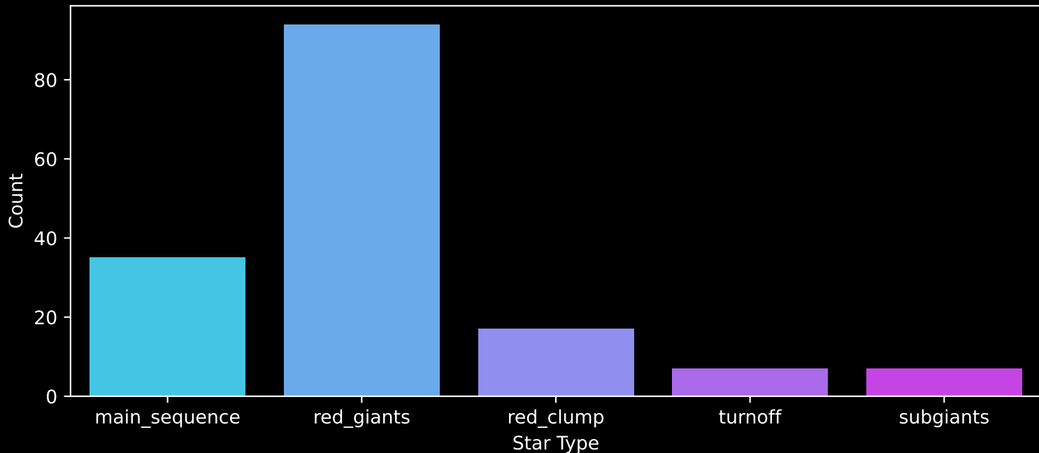
APOGEE DR17 Field: [200+22_MGA] Count plot of Star Type
