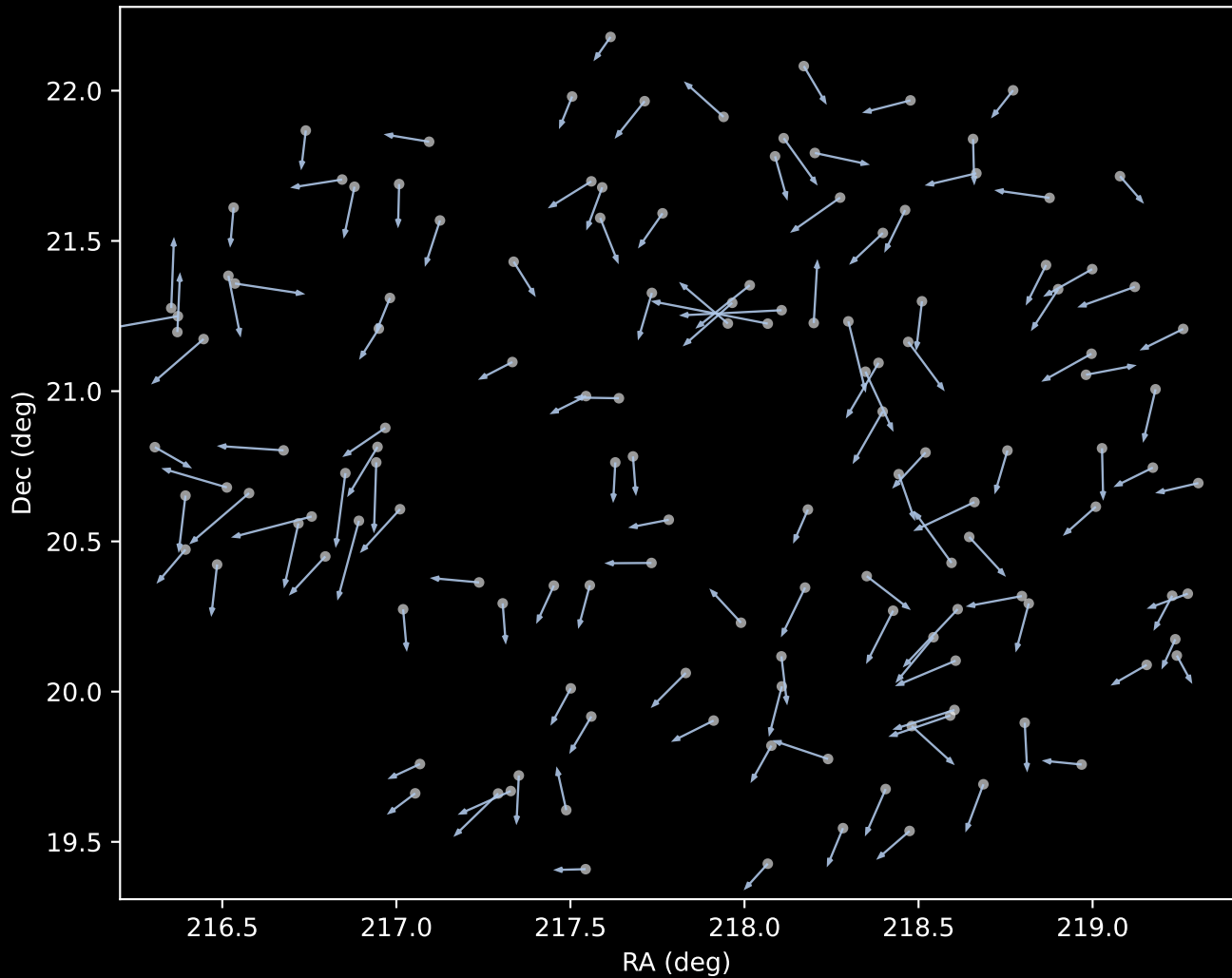
APOGEE DR17 Cluster 1 Proper Motion Vectors (n=136)
