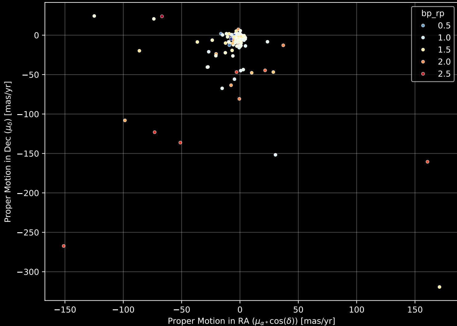
APOGEE DR17 Field: [200+22_MGA] Proper Motion Diagram (n= 160)
