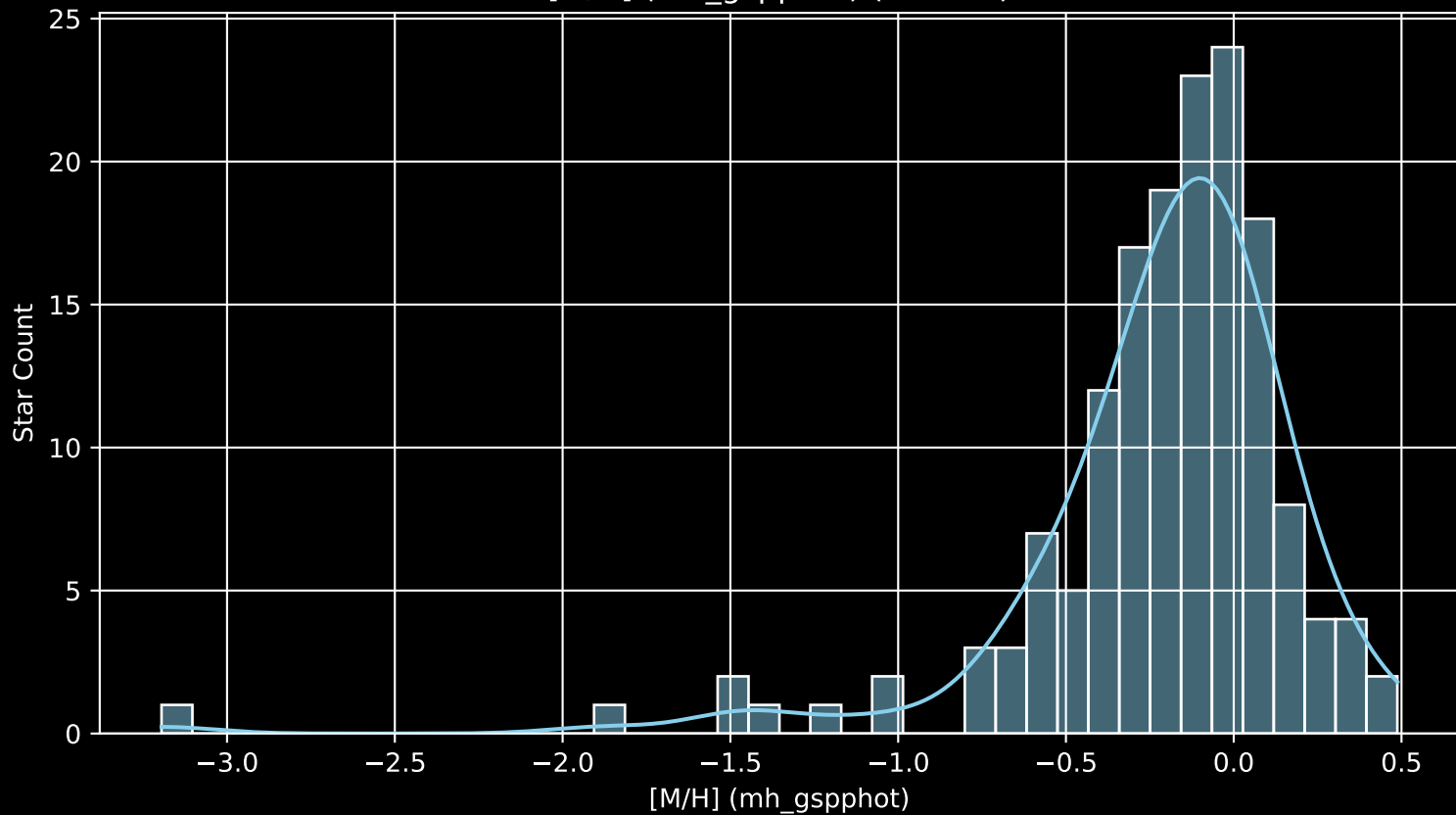
APOGEE DR17 Field: [200+22_MGA [M/H] (mh_gspphot) (n= 157)
