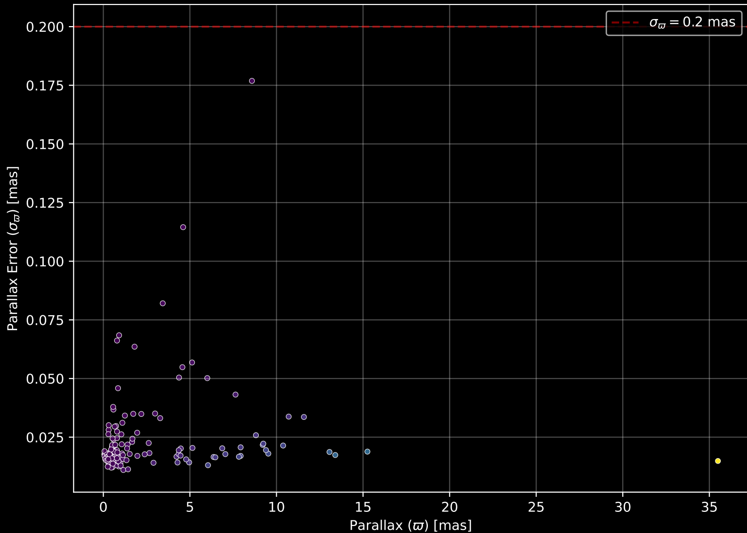
APOGEE DR17 Field: [200+22_MGA] Parallax Quality (n= 160)
