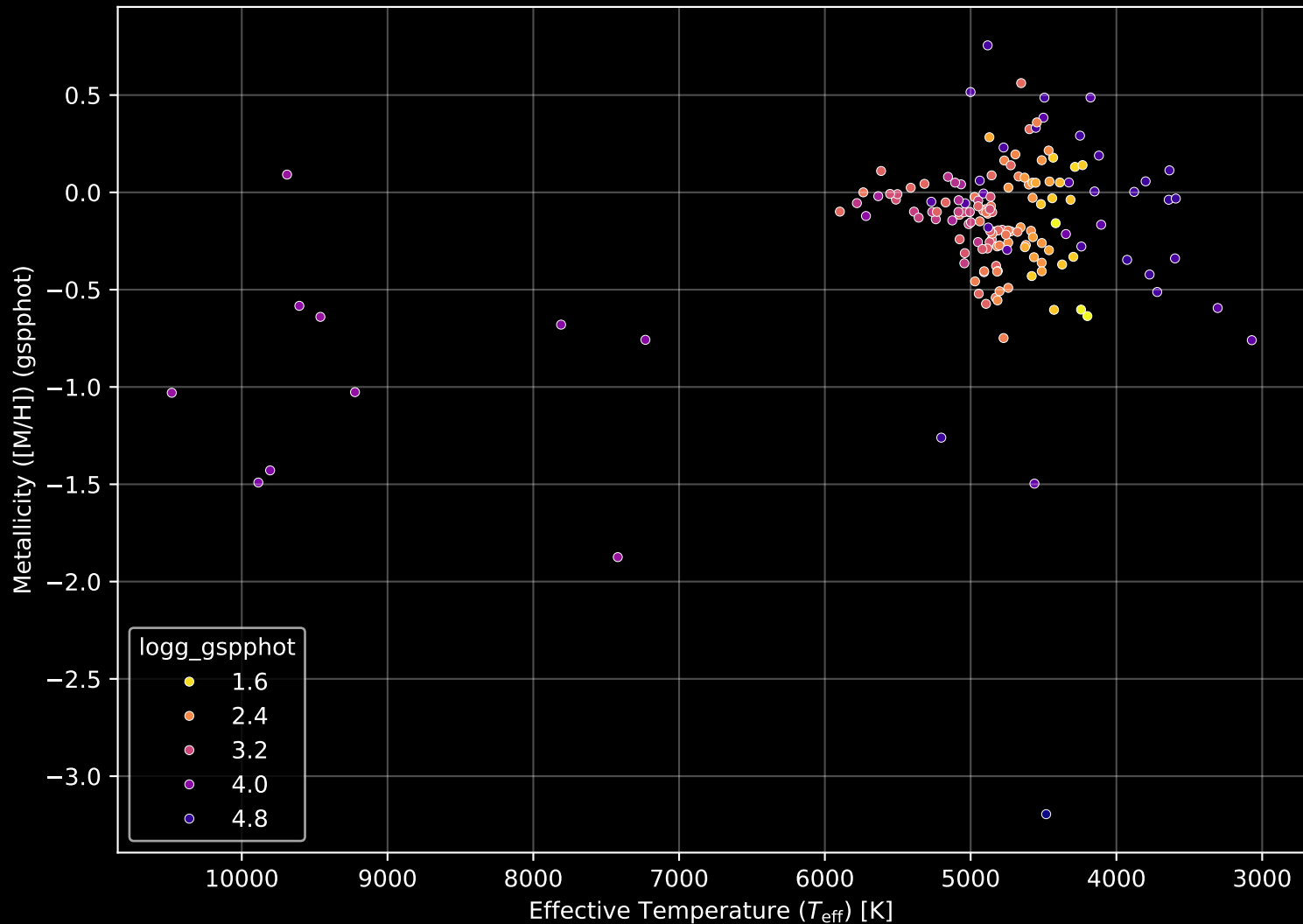
APOGEE DR17 Field: [200+22_MGA] Stellar Population Parameters (n= 160)
