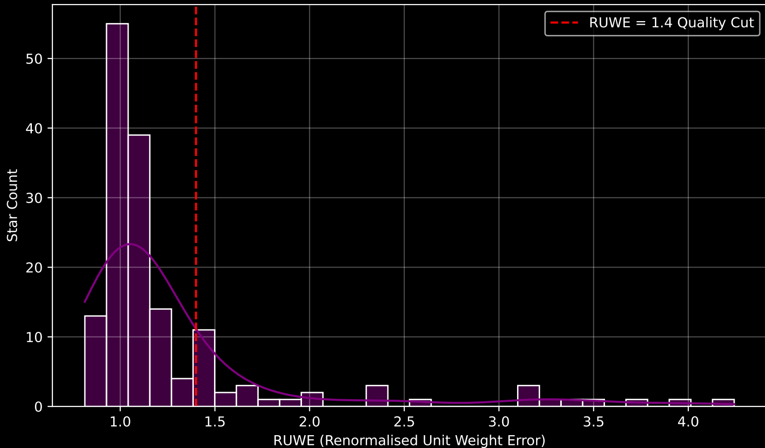
GAPOGEE DR17 Field [200+22_MGA] RUWE Distribution (n= 158)
