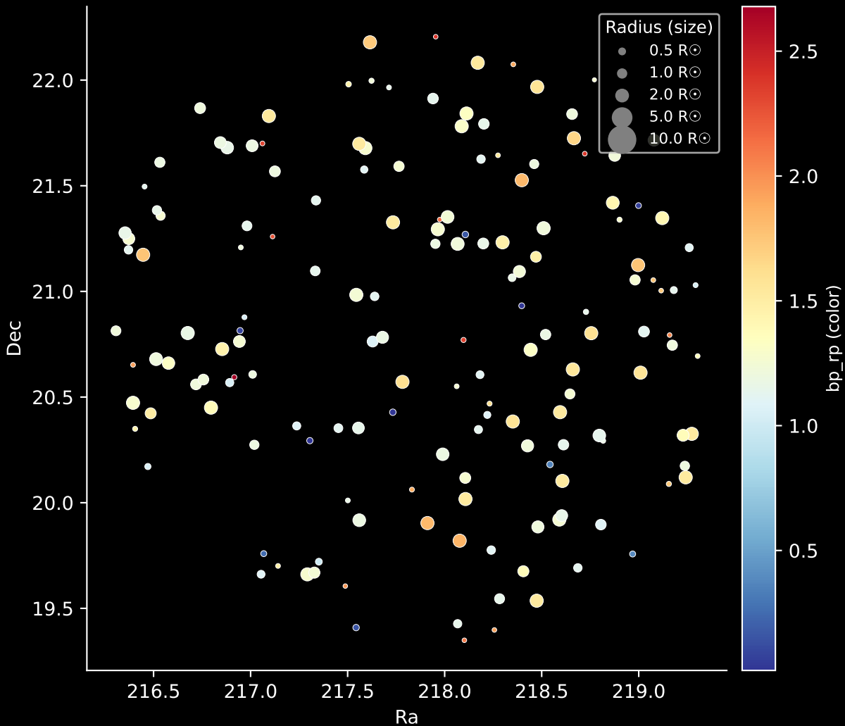
APOGEE DR17 Field: [200+22_MGA] Stars: 160
